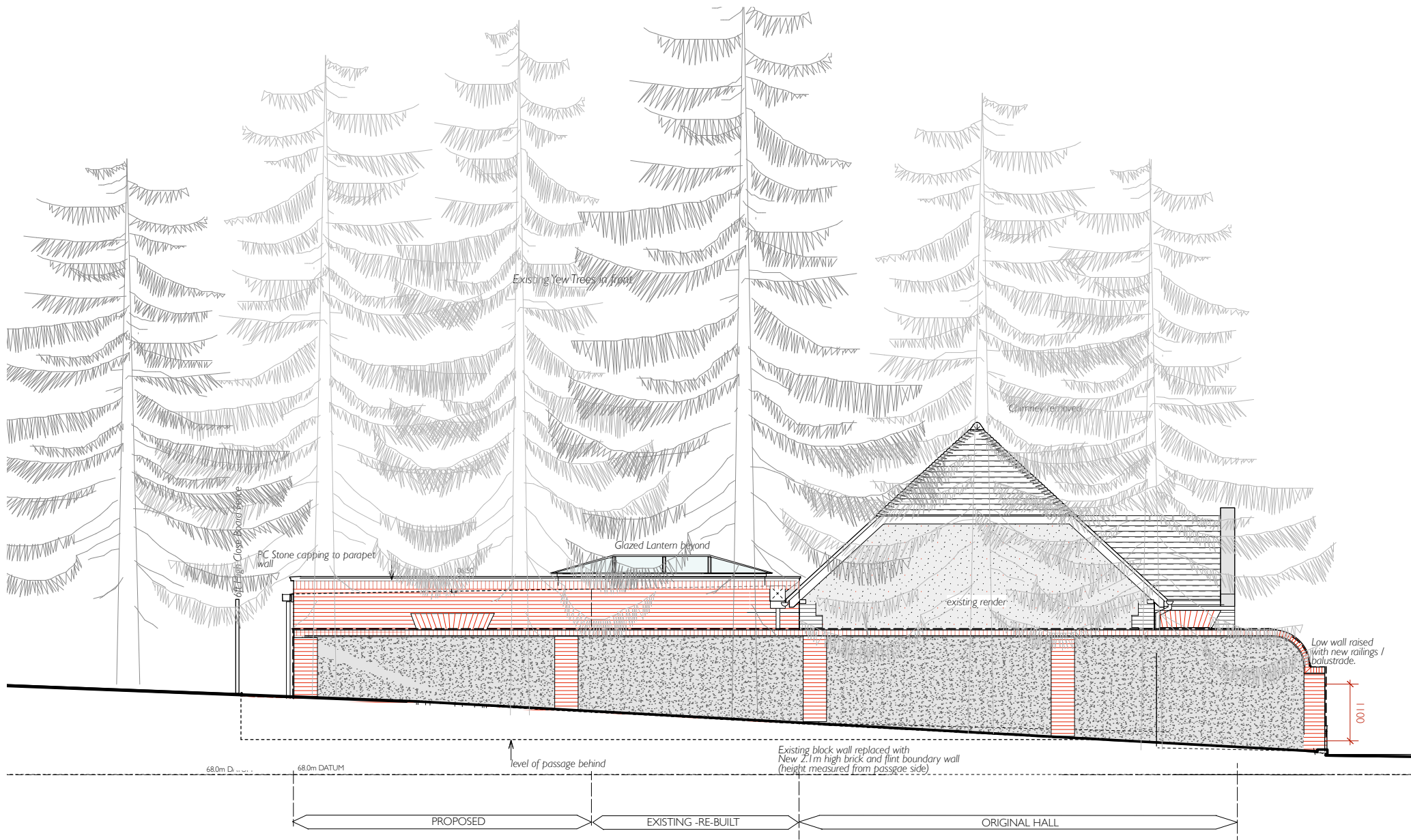
SOUTH ELEVATION TO NEW BOUNDARY WALL
