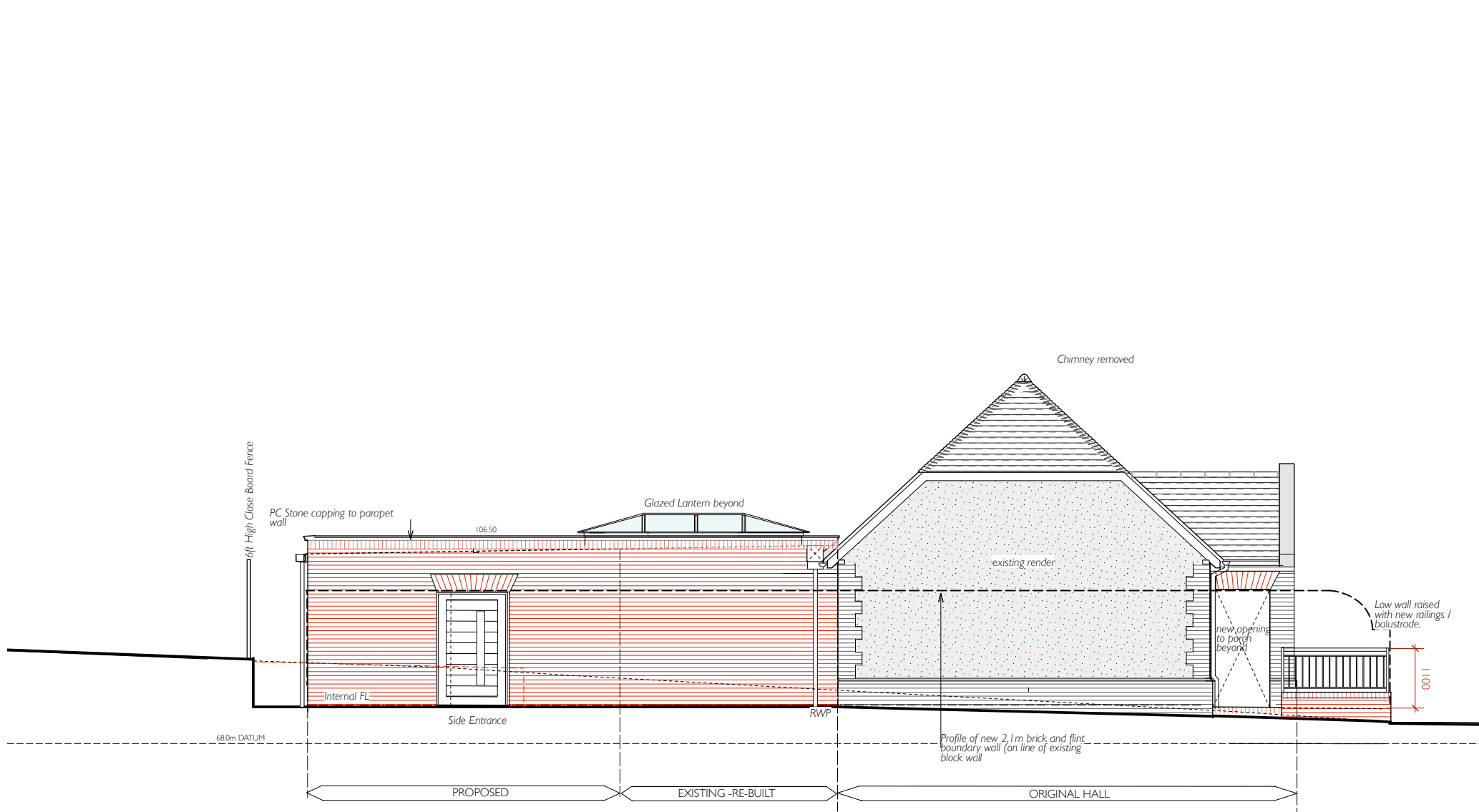
SOUTH ELEVATION
