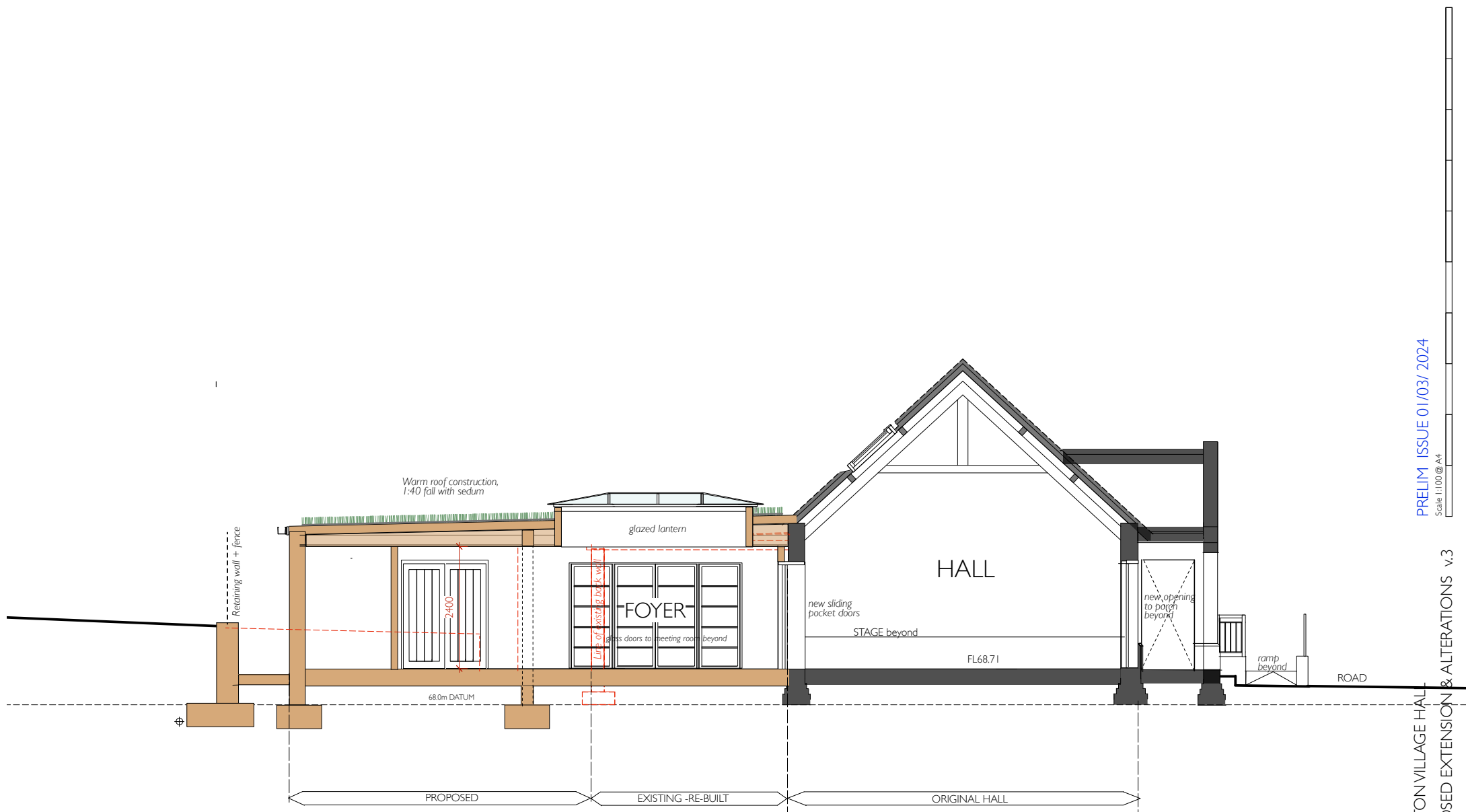
SECTION A
