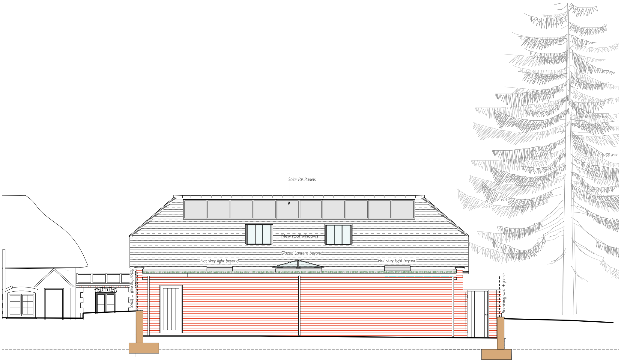
WEST ELEVATION
